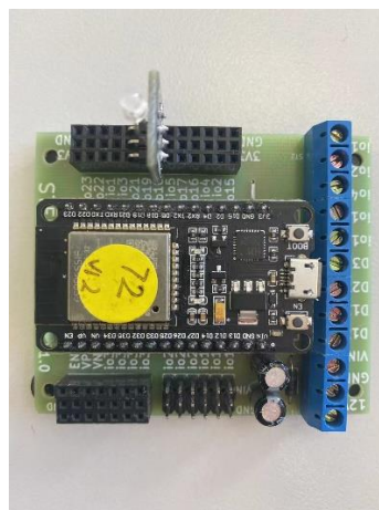
Figure 4 Top view connection on E32W
